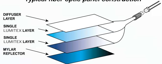
Typical fiber optic panel construction
